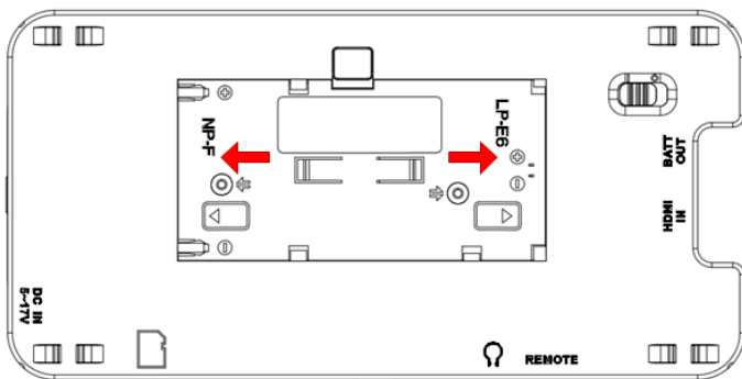
Figure 3-2 Battery Installation
