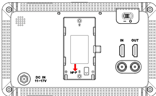
Figure 3-1 Battery Installation
