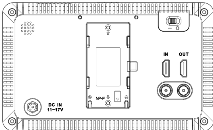
Figure 7.2-2 Back View(Unit: mm)
