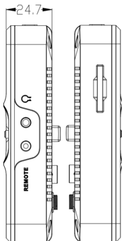
Figure 7.2-3 Side View(Unit: mm)
