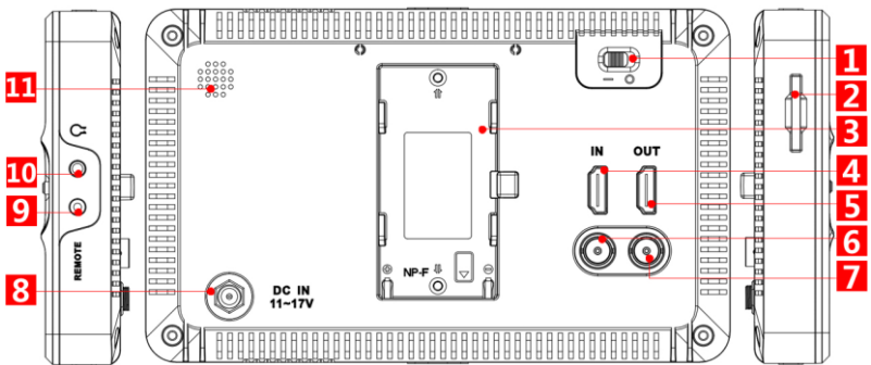
Figure 4.1-1 Parts in Rear Panel
